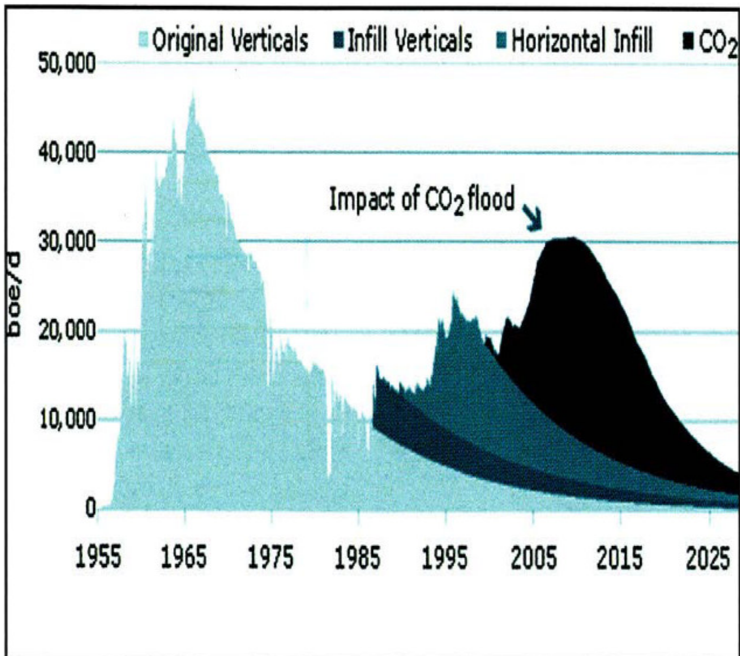
Figure 1: Historical production from the Weyburn field, and the impact of carbon dioxide (CO 2 ) flood Courtesy EnCana
